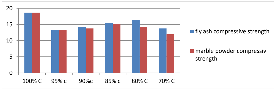
Fig 1: comparison of compressive strength of fly ash concrete and marble powder concrete at 7Days
