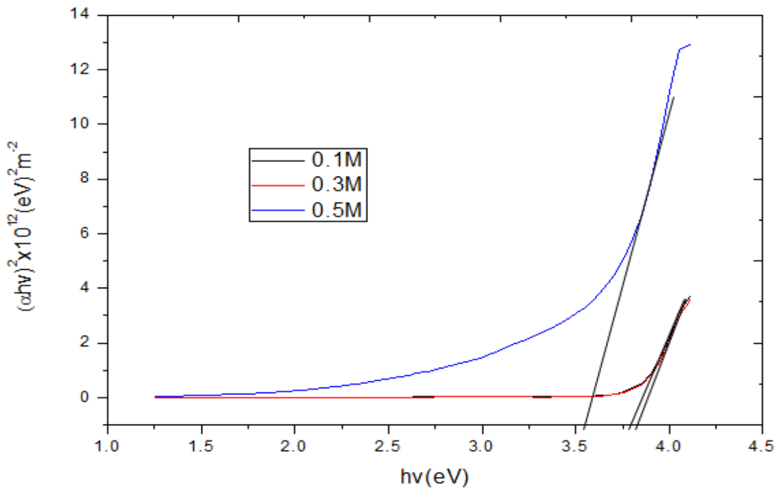
Fig.9: Plot of (\alpha hv)^2 against h\nu at different concentrations for 333K
