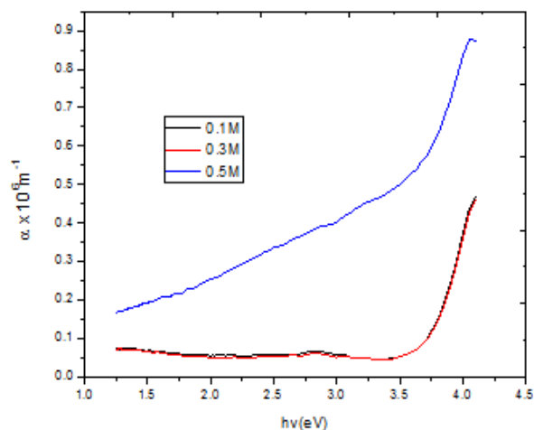
Fig. 7: Plot of \alpha against h\nu at different concentrations for 333K
